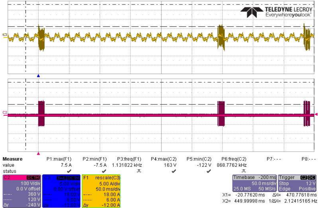
Actual Test CS117 Waveform #3 at 1MHz, 3 Bursts +360V/6A, on Power Line 1
