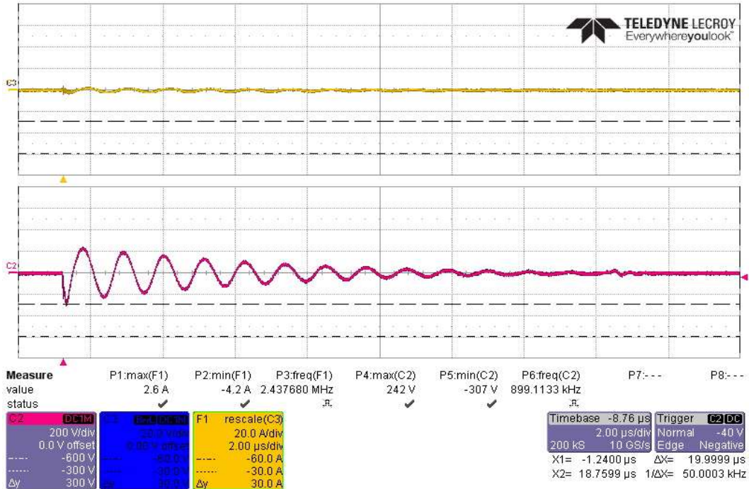
Actual Test CS117 MS Waveform #3 at 1MHz, Subsequent Transient -300V, on PV Bundle
