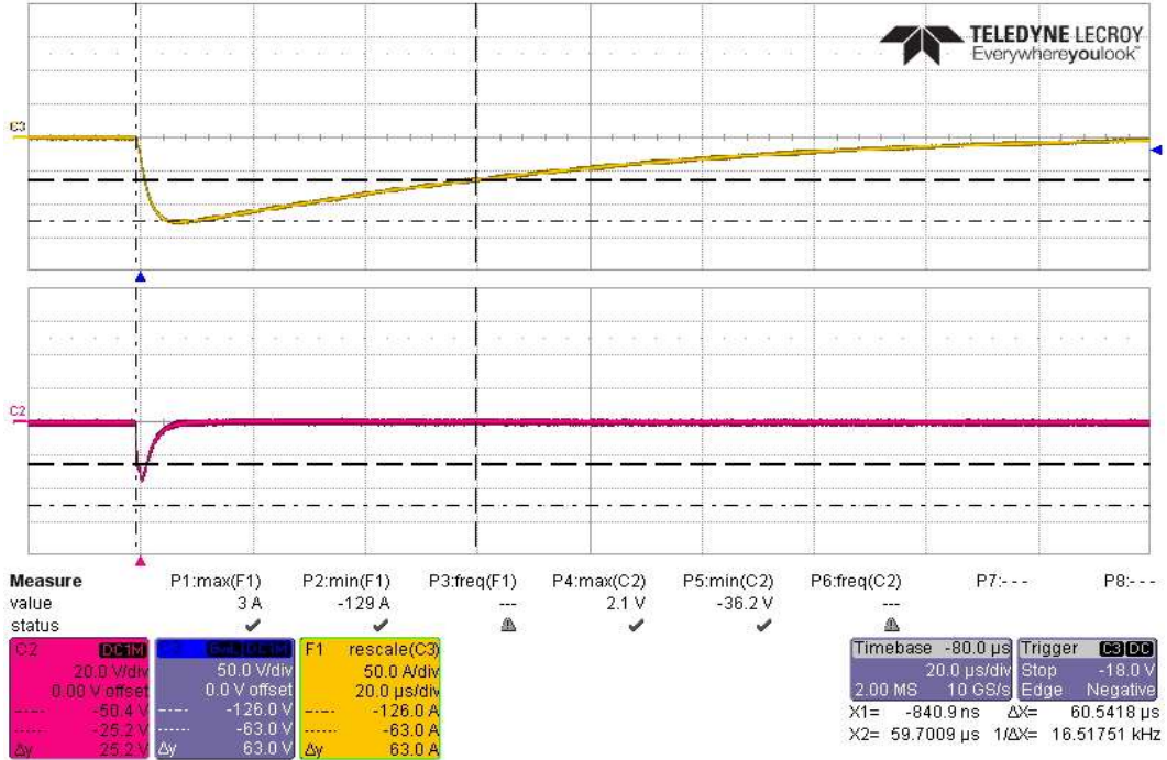
CS117 Current Verification Waveform #1, First Transient -120A, T2
