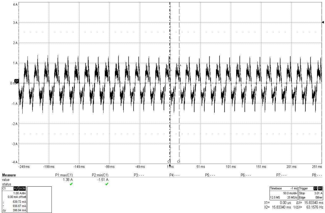
Actual CS116 Damped Sinusoidal Transient Test at 100 MHz on AC L1
