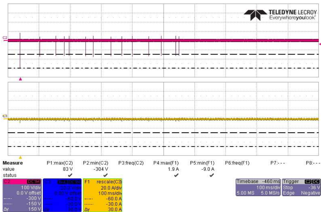
Actual CS117 Voltage Waveform #2 Test, 14 Transient -300V/60A & -150V/30A on PV Return Side
