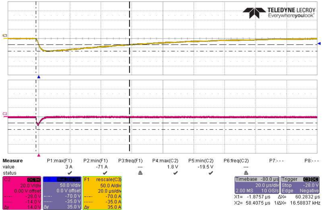
CS117 Current Verification Waveform #1, Subsequent Transient -60A, T2
