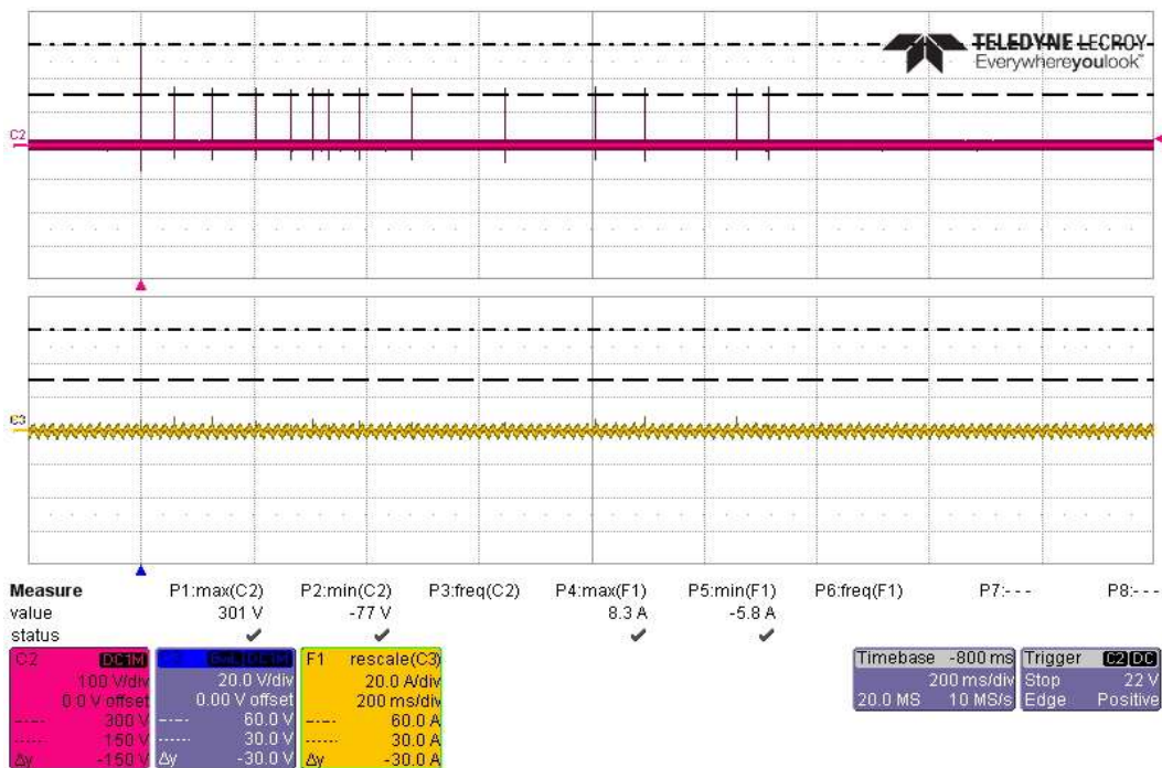
Actual CS117 Voltage Waveform #2 Test, 14 Transient +300V/60A &amp; +150V/30A on AC High Side
