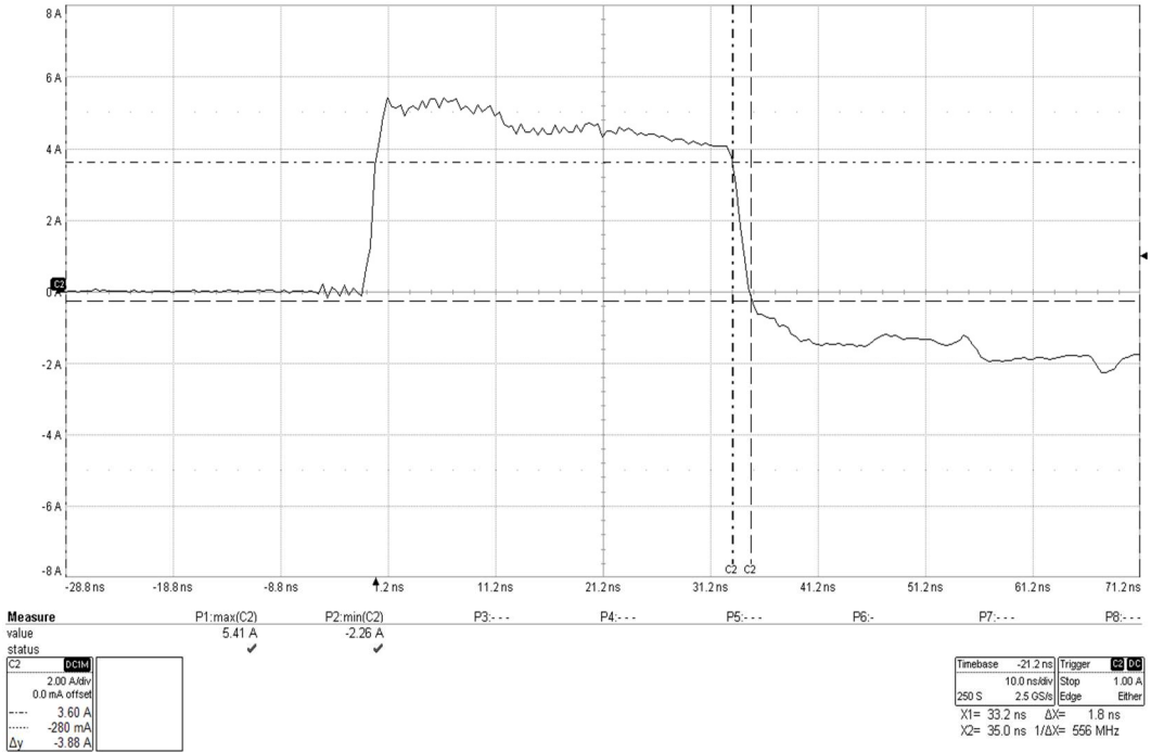
CS115 Verification Fall Time
