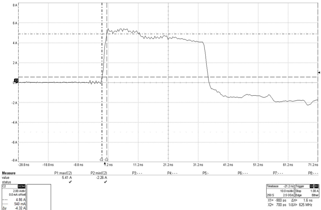
CS115 Verification Rise Time
