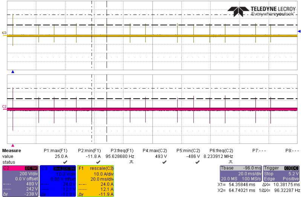
CS117 Current Verification Waveform #3 at 10MHz, 14 Transients +24A/12A
