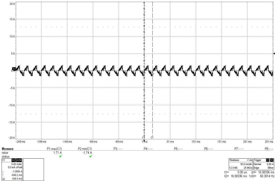
Actual CS116 Damped Sinusoidal Transient Test at 1 MHz on AC L2
