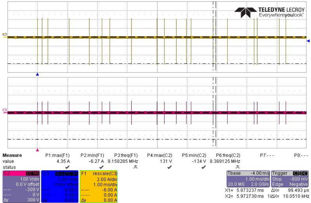
CS117 Current Verification Waveform #3 at 10MHz, 20 Transients at -6A
