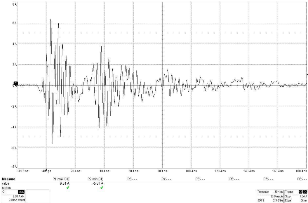
CS115 Test on AC L2
