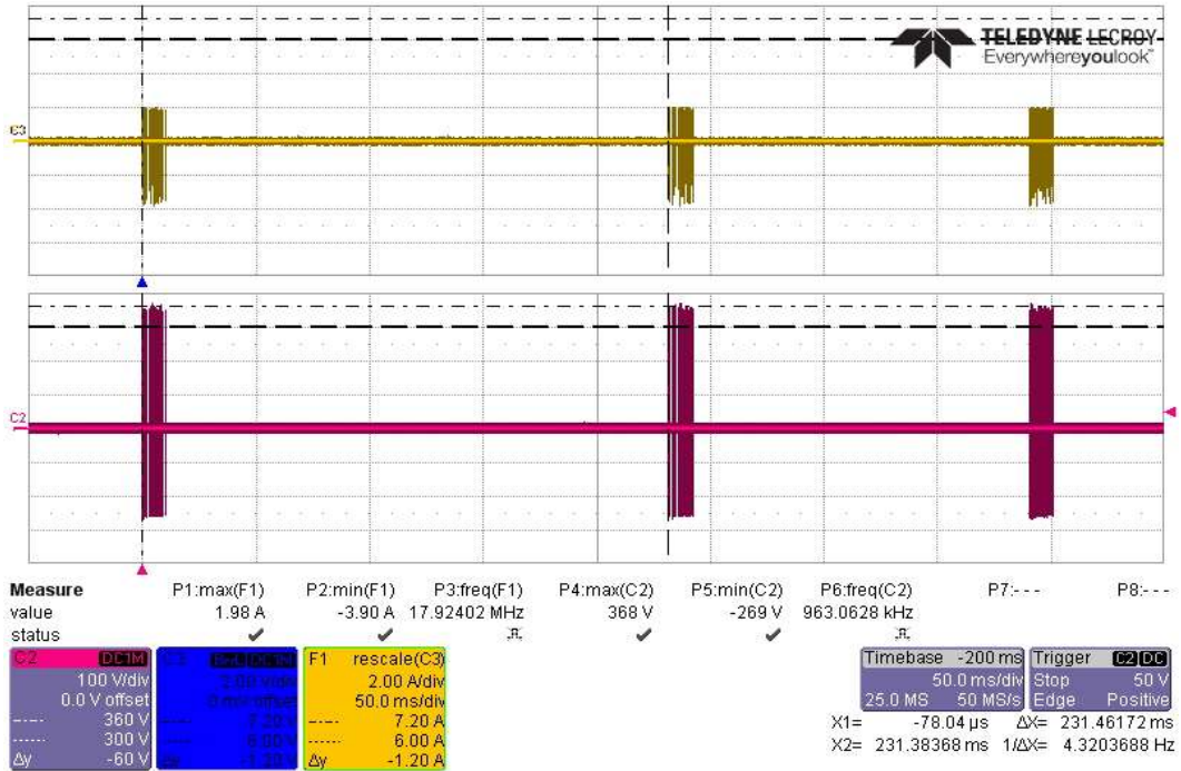
CS117 Voltage Verification Waveform #3 at 1MHz, 3 Bursts at +360V
