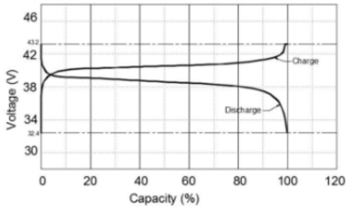
Charge & Discharge curve with 1.0C @ 25°C
